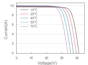
Current-Voltage Curve JAM60S01-300/PR
